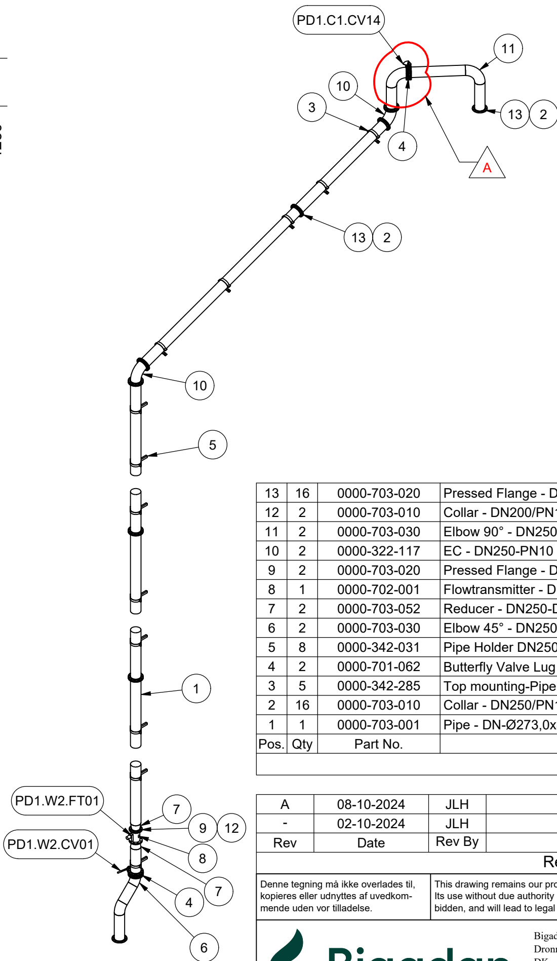
Parts List
